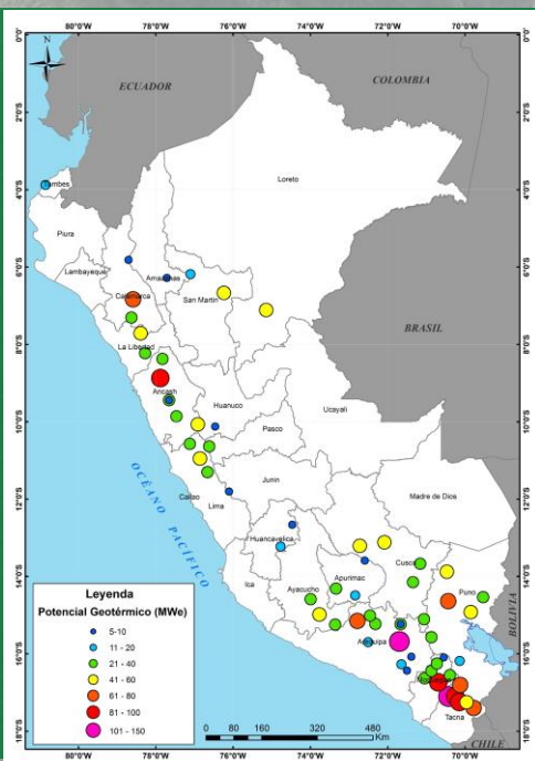
Figure 1: Map of the Geothermal Areas in Peru Gobierno del Perú (www.gob.pe)
